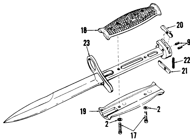
BAYONET - KNIFE M7
