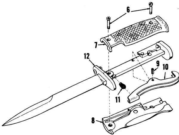
BAYONET - KNIFE M5
