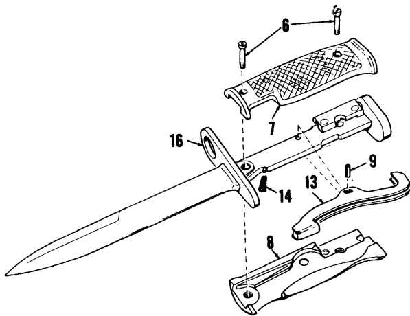
BAYONET - KNIFE M6
