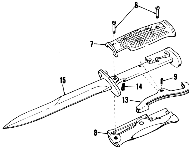
BAYONET - KNIFE M5A1
